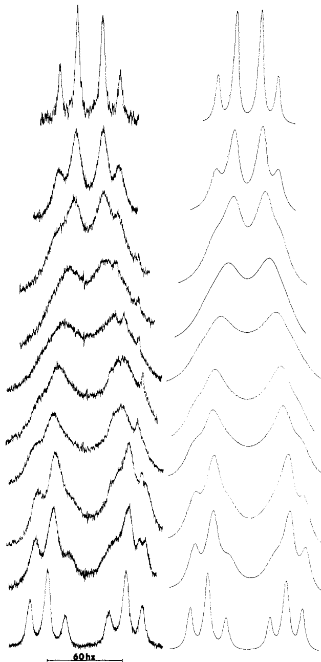
Figure 5. The observed (left) and calculated 90-MHz spectra of the \alpha protons of thiane-3,3,5,5- d_4 -1-( N -tosyl)imide 1-oxide ( 8 ) in \text{CHCl}_3 as a function of temperature. There is a small impurity peak at the extreme right of the observed spectra. From top to bottom, the temperatures and the mean lifetimes ( k^{-1} in seconds) for both isomers are +27 (fast exchange), -45 (0.00165, 0.00085), -51 (0.0039, 0.0020), -54 (0.0070, 0.0036), -58 (0.0110, 0.0057), -62 (0.0175, 0.0089), -65 (0.024, 0.0120), -67.5 (0.038, 0.019), -70 (0.059, 0.030), and -89 (slow exchange).
